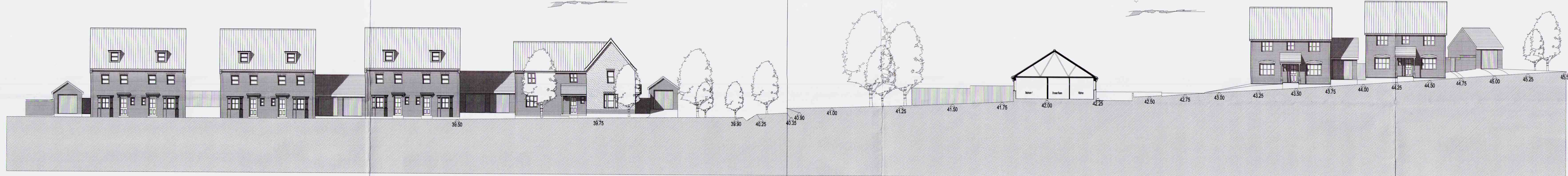
Street Elevation ( Site Section ) 10-10
