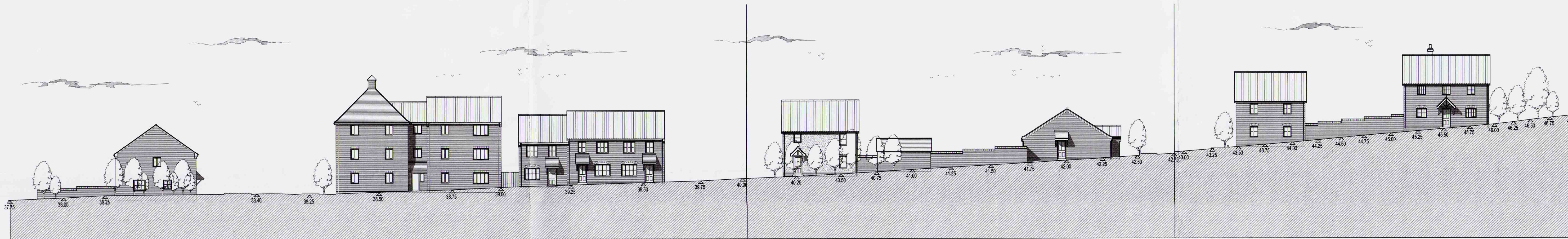
Street Elevation ( Site Section ) 4-4
