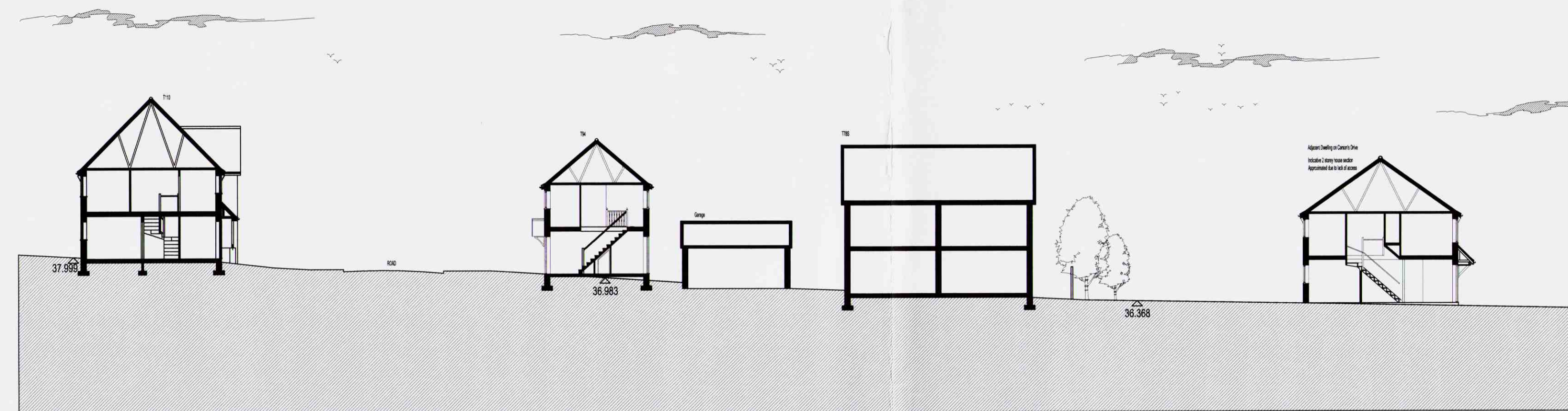
Site Section 13-13
